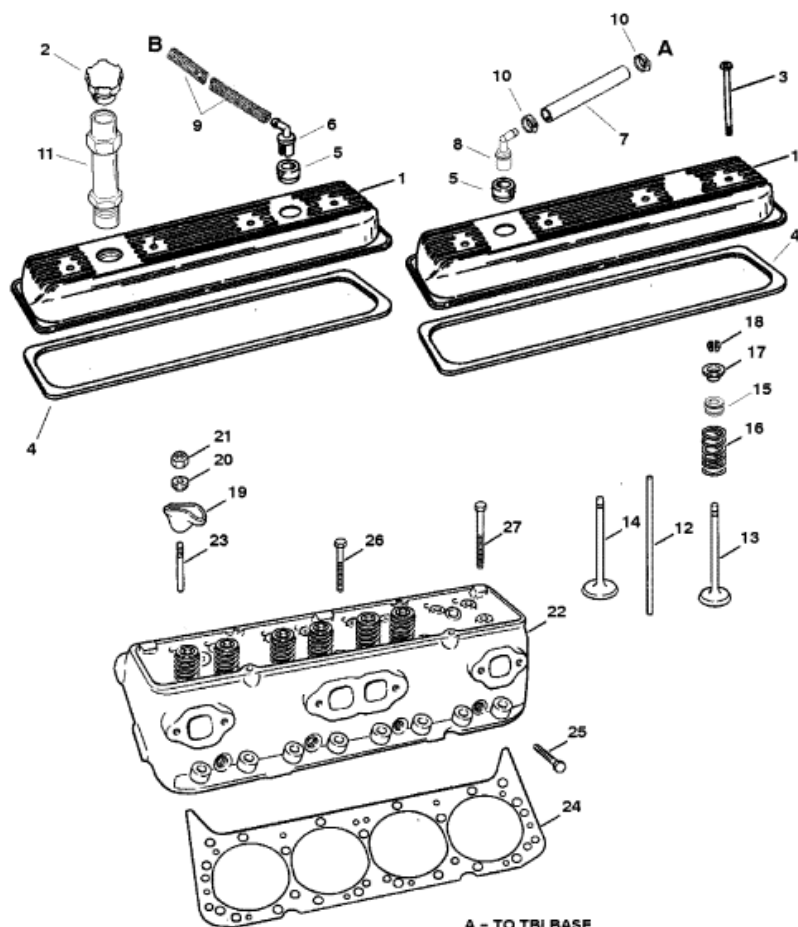
A = TO TBI BASE B = TO FLAME ARRESTOR
